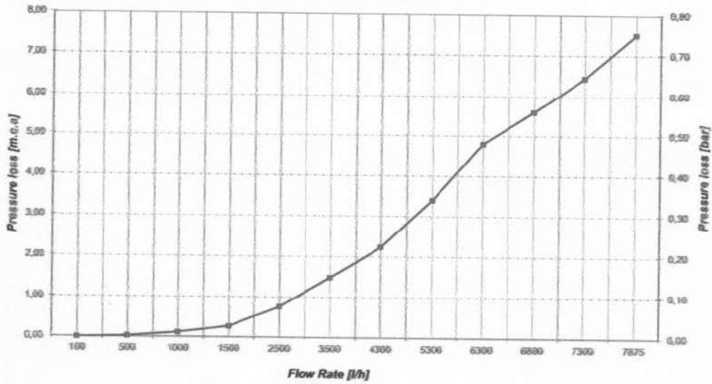
LAQUAM Q 3 6,3 DN25x260 (G 1 1/4" B)
